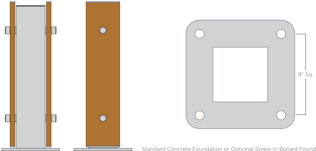
Standard Concrete Foundation or Optional Screw-In Bollard Foundation (1)
