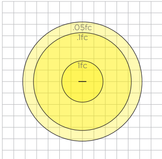
AURA-LNR-D-6-L35SO Mounted at 10'
