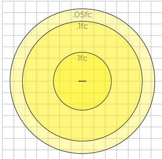
AURA-LNR-D-12-L35SO Mounted at 10'
