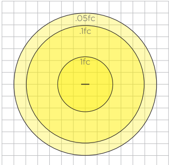
AURA-LNR-D-10-L35SO Mounted at 10'
