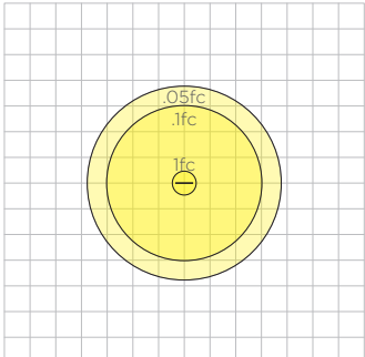
AURA-LNR-D-2-L35SO Mounted at 10'
