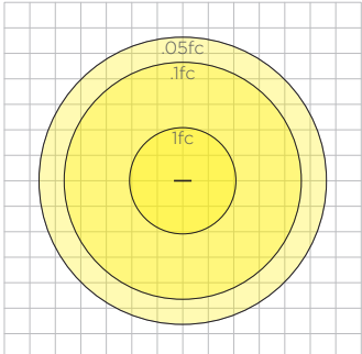
AURA-LNR-D-8-L35SO Mounted at 10'
