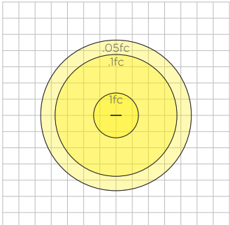
AURA-LNR-D-4-L35SO Mounted at 10'
