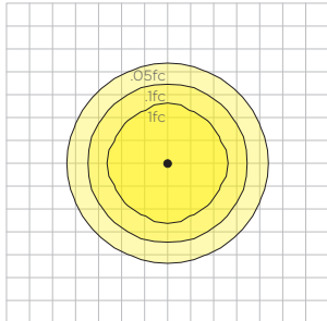
STELA-L30HO-20 10' AFG BUG Rating: B3-U0-G0
