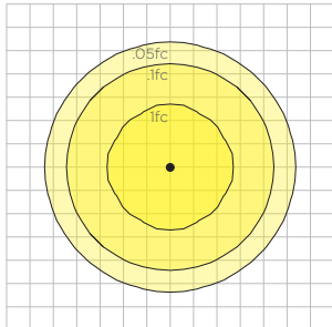
STELA-L30HO-30 10' AFG BUG Rating: B3-U0-G0
