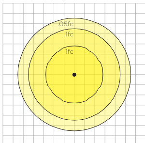
PIKE-L30HO-40 10' AFG BUG Rating: B3-U0-G0
